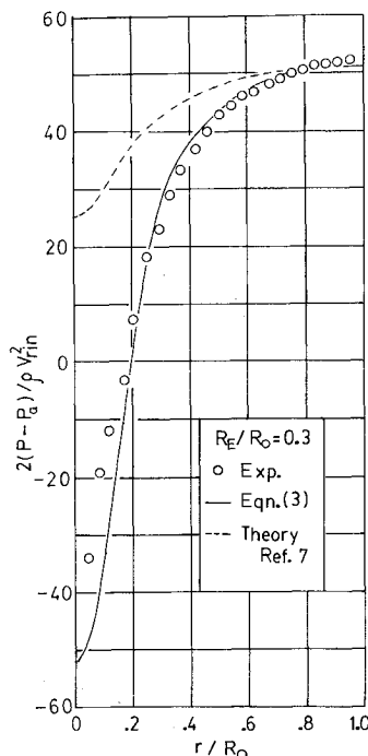
Fig. 2 Radial distribution of the static pressure.
