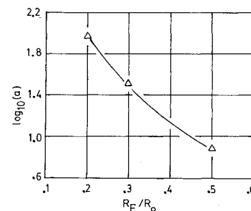
Fig. 3 Variation of parameter a with the contraction ratio.
